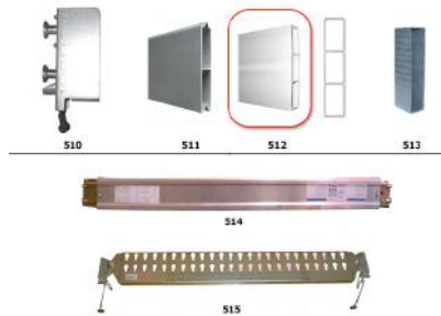
FORKLIFT BARRIER 400 MM. PART NUMBER | 11171000569
