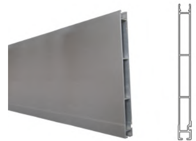
DROP SIDE AL. PROFILE (LOWER) PART NUMBER | 11090139405
