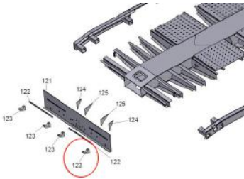
RAMP CONNECTING BRACKET PART NUMBER | 10109001661
