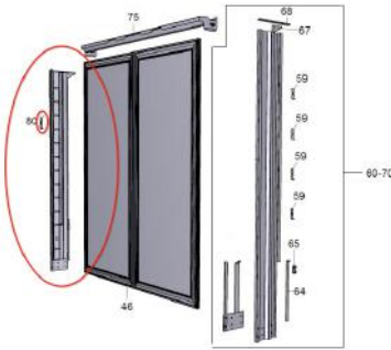
REAR DOOR HINGE PART NUMBER | 11253000018
